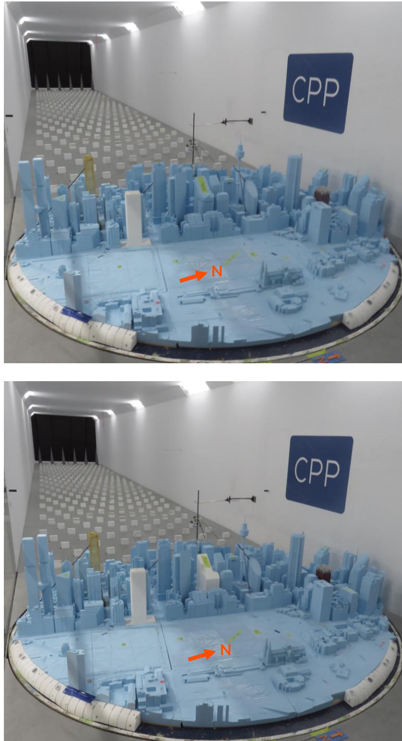
Figure 1a: Photographs of Wind Tunnel Test and Surrounds Model – Configuration A (top) and Configuration B (bottom).
